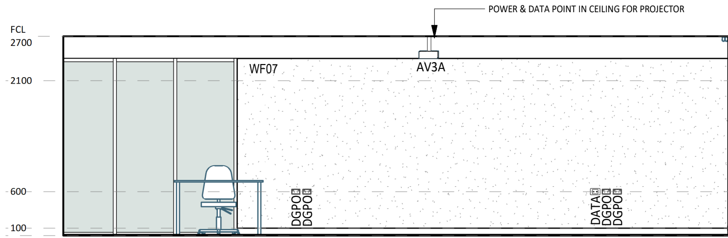
2 ELEVATION DETAIL 60-043 1 : 50
