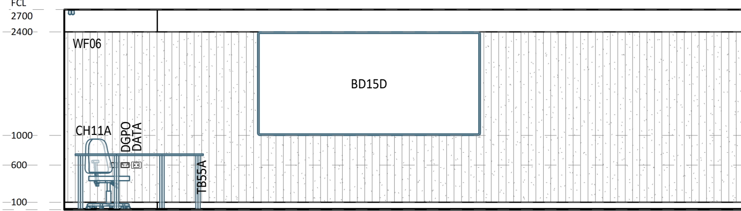
4 ELEVATION DETAIL 60-043 1 : 50
