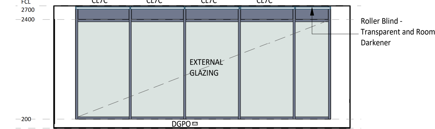
3 ELEVATION DETAIL 60-043 1 : 50
