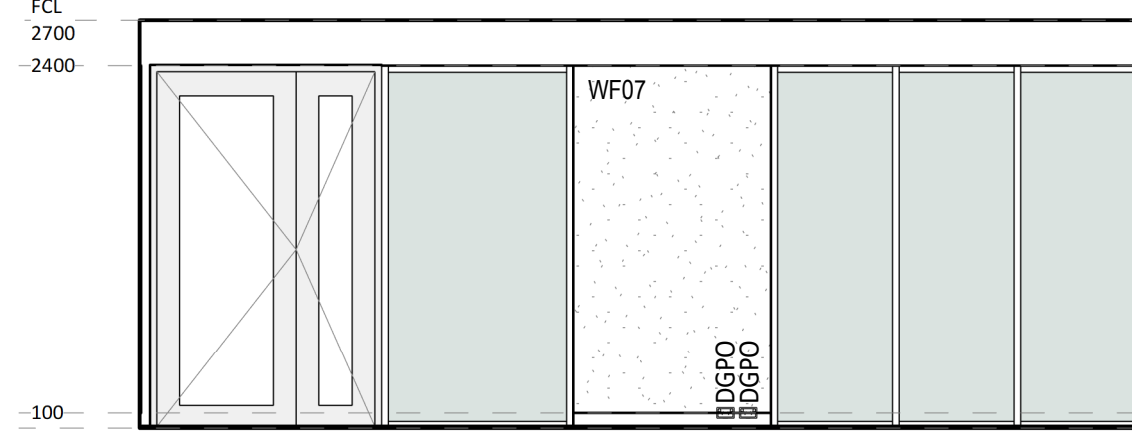
5 ELEVATION DETAIL 60-043 1 : 50
